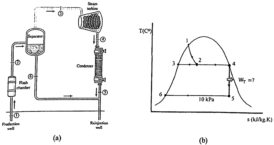
Figure 2. (a) Schematic of geothermal steam power plant, and (b) corresponding TS-diagram.
