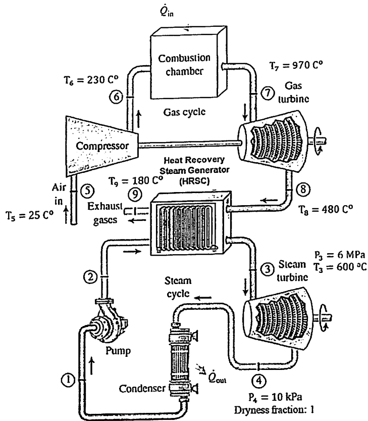
Figure 1. Schematic of the combined gas-steam power plant.
